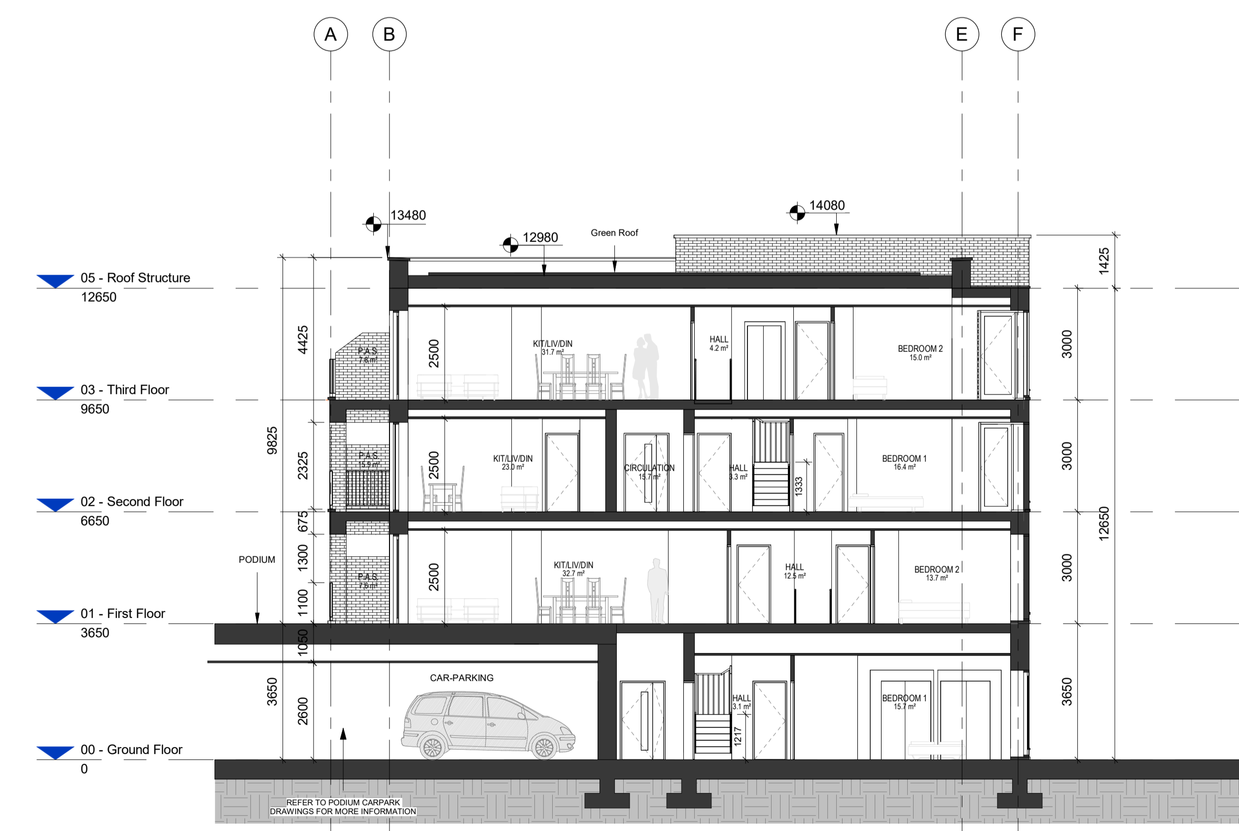
2 Section BB' 1: 100
