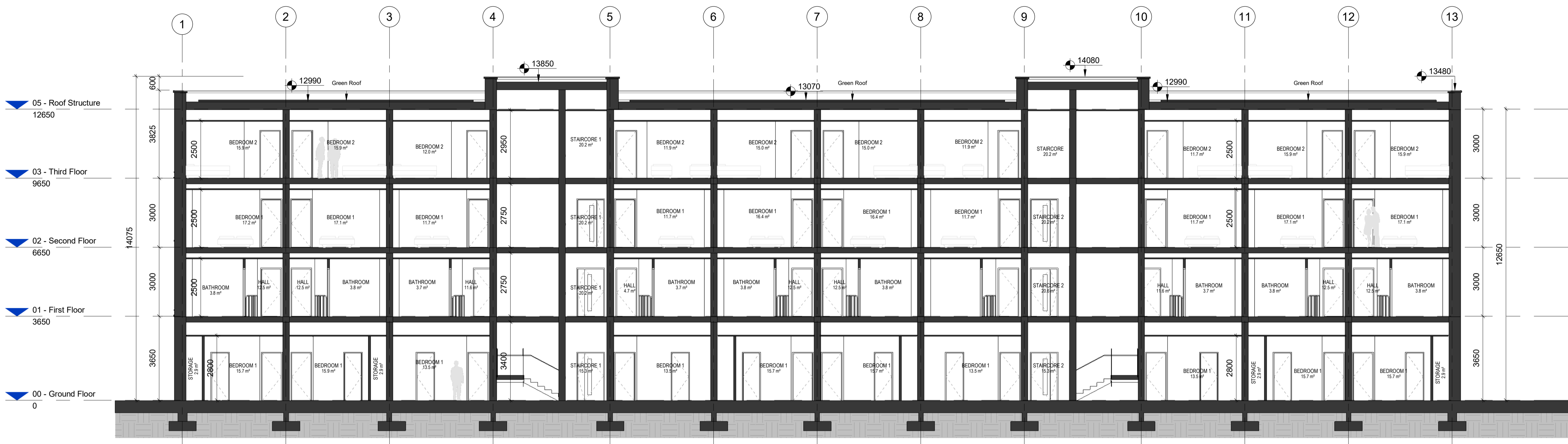
1 Section AA' 1: 100
