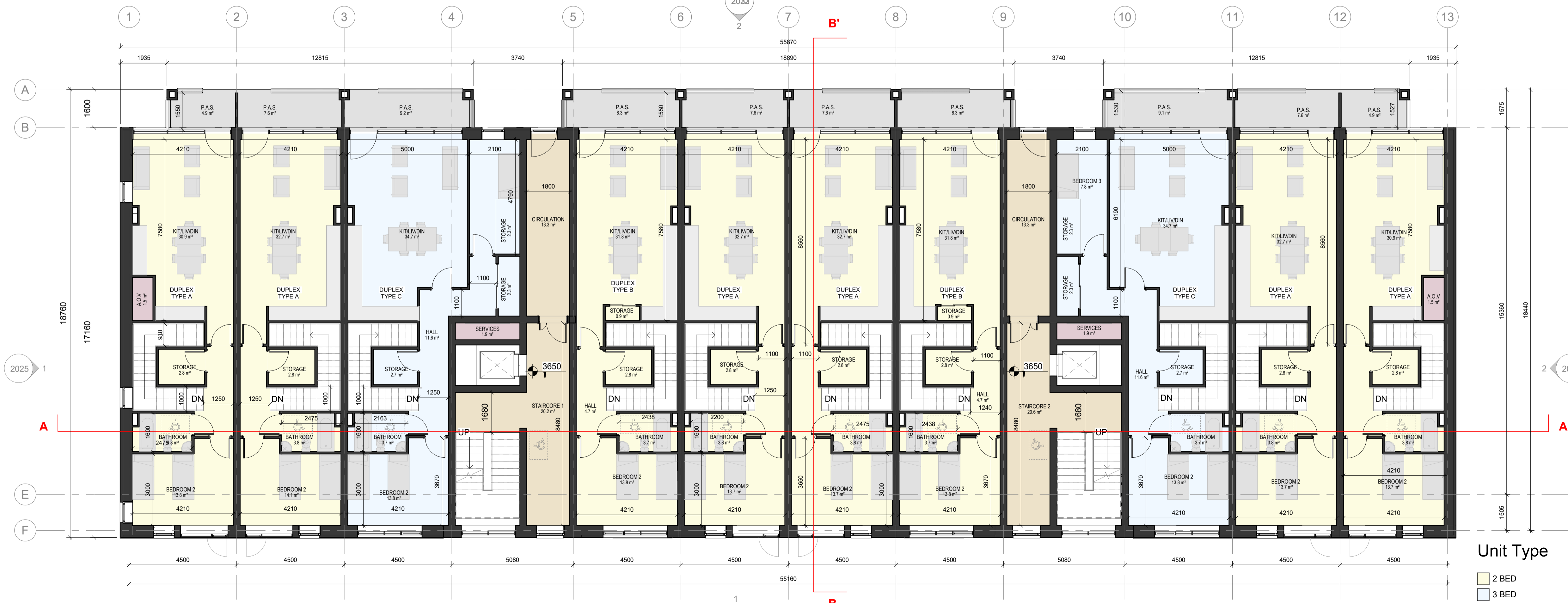
2 First Floor 1:100
